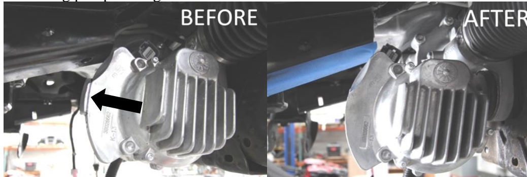
Figure 13: Power Steering Casting cut.
