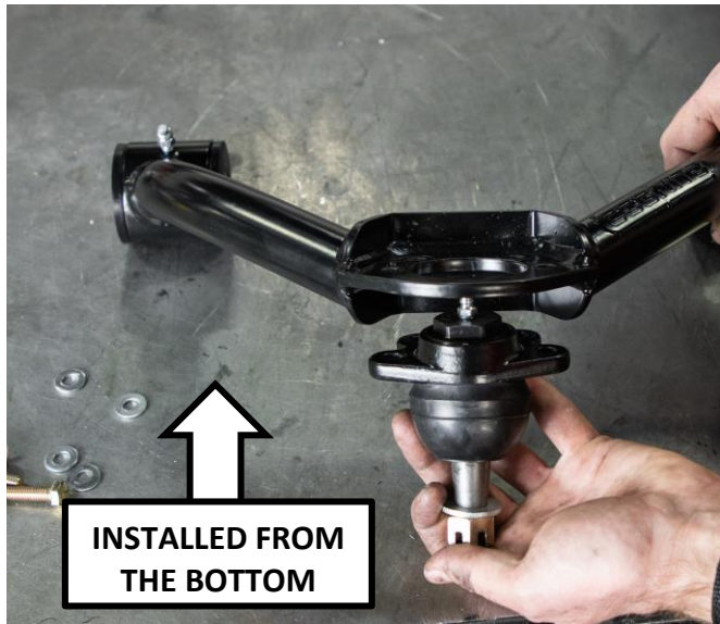
Figure 4: Bolt-in Ball Joint Installation
