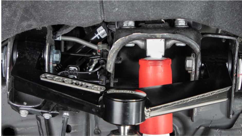
Figure 7: Cognito UCA Installation
