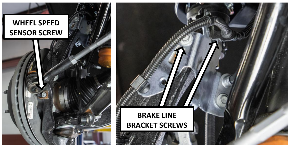
Figure 3: Wheel Speed Sensor and Brake Line Bracket Removal
