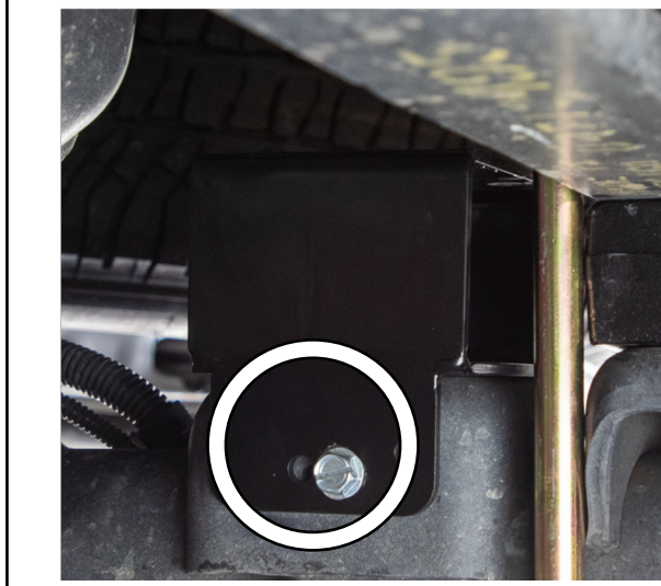
Figure 61: Rear Bump Stop Installed Front Side
