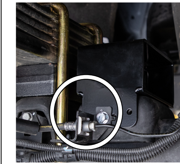
Figure 60: Rear Bump Stop Installed Rear Side
