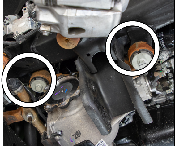
Figure 23: Driver Side Differential Mounting
