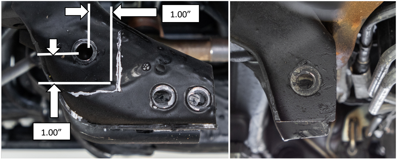
Figure 25: Trim Rear Crossmember
