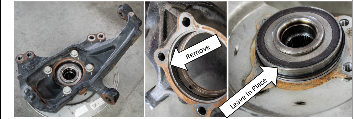
Figure 48: Disassemble Hub Assembly
