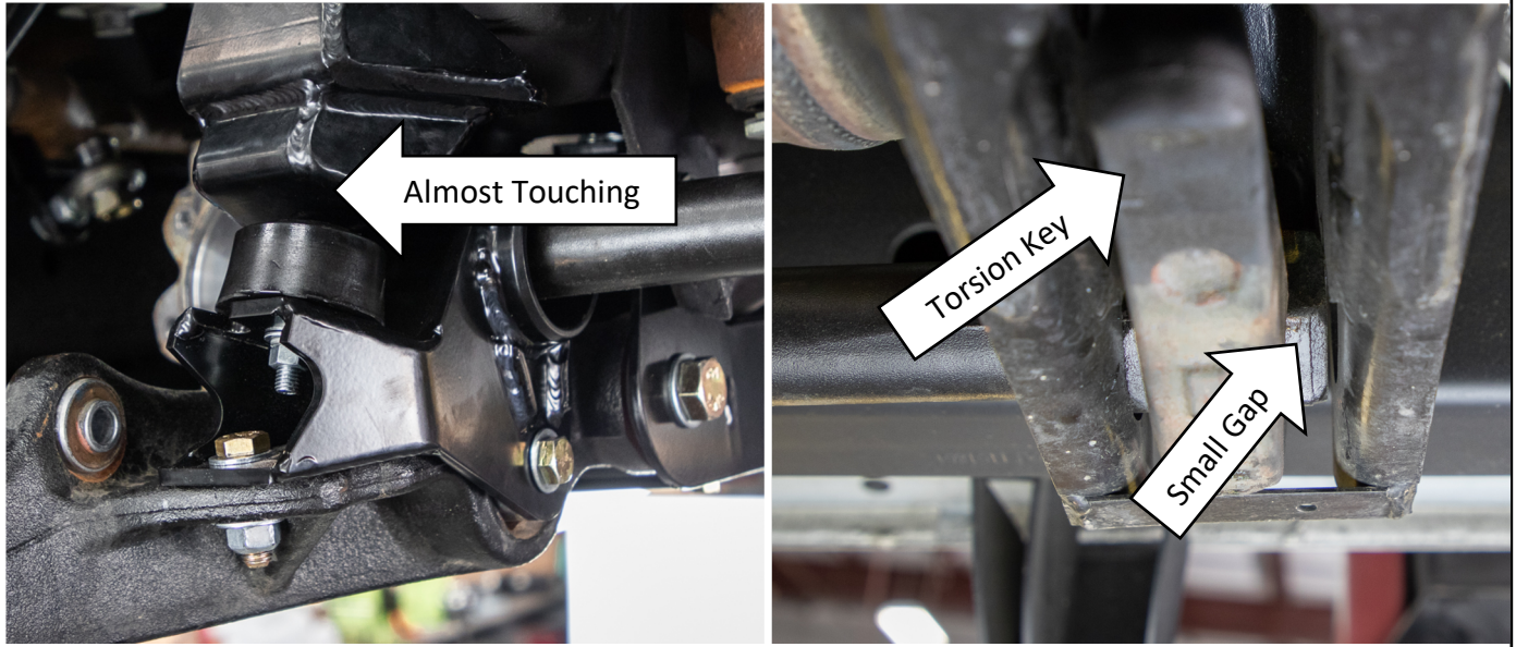
Figure 47: Reinstall Torsion Bars
